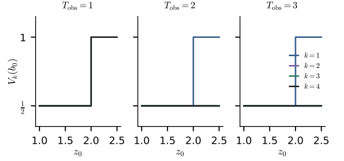
Figure 1: The closed-form values of Proposition 5 on the delayed grid: flat at \frac{1}{2} while a branch falls, jumping by exactly \frac{1}{2} at z_0 = 1 + \min(k, T_{\text{obs}}) , constant beyond.
